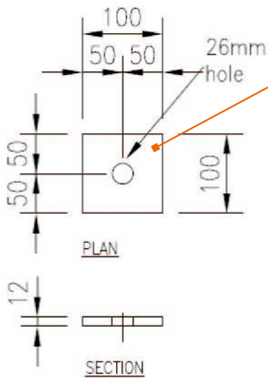
Plate Washer PW2
