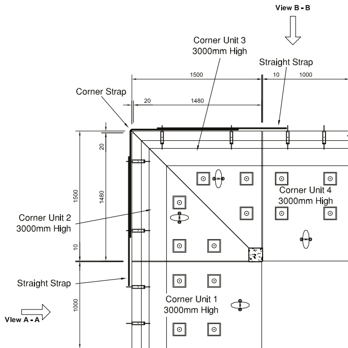
Corner Section Plan
